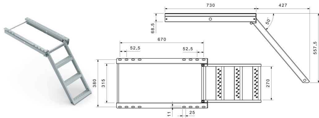
3 BASAMAKLI MERDİVEN / 3 STEPS LADDER
