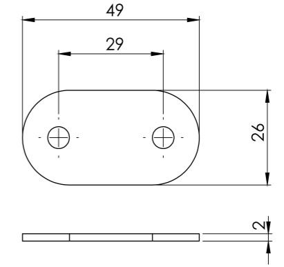
BRANDA TOKA SABİTLEME PULU KROM - GALVANİZ BUCKLE BRACKET WASHER (SS) - (ZP)
