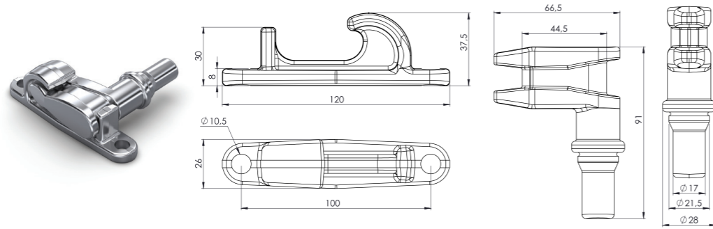
UNITNOVA TEK YÖN KANCA TAKIMI Ø22 CAM AND KEEPER FOR LOCK Ø22 (SS)
