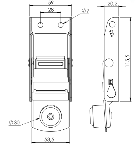
KÜÇÜK BRANDA TOKASI TAKOZLU KROM - GALVANİZ SMALL WEDGED TARPAULIN BUCKLE (SS) - (ZP)
