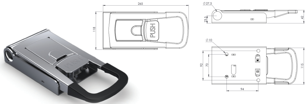
KÜÇÜK DIŞTAN KİLİT GALVANİZ Ø27 SMALL PUSH HANDLE LOCK WITH KEY Ø22 (ZP)
