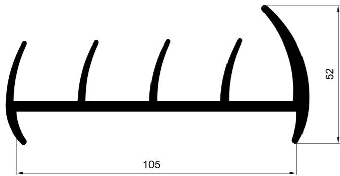
LP 105MM KAUÇUK PROFİL / RUBBER PROFILE 105MM
