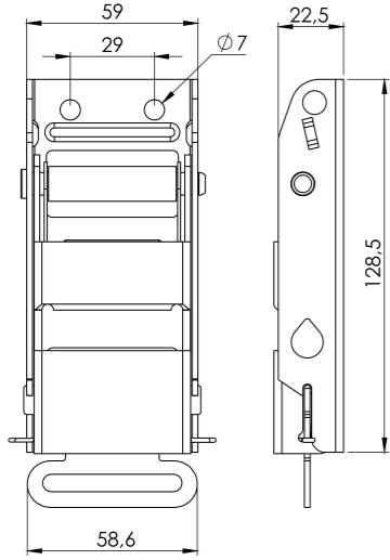
BRANDA TOKASI KİLİTLİ KROM TİP1 TARPAULIN BUCKLE WITH LOCK TYPE1 (SS)
