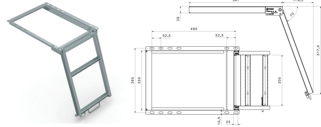
ECOSERIES 2 BASAMAKLI MERDİVEN DALDIRMA GALVANİZLİ ECOSERIES 2 STEPS LADDER HOT DIP GALVANIZED
