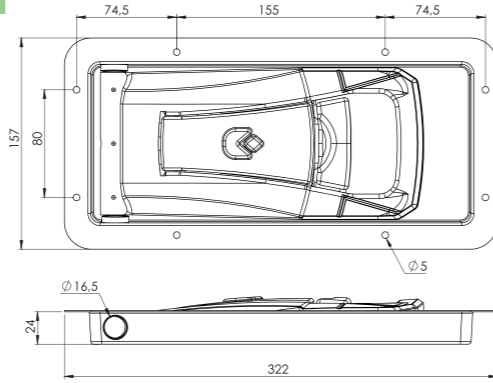
UNITNOVA GÖMME KİLİT 24MM KROM Ø16 UNITNOVA RECESSED DOOR LOCK WITH KEY 24 MM Ø16 (SS)
