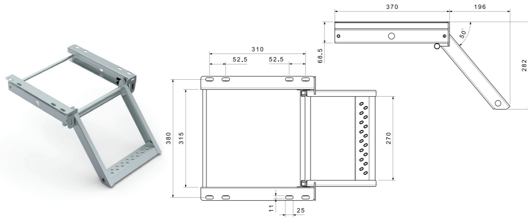
TEK BASAMAKLI MERDİVEN / SINGLE STEP LADDER
