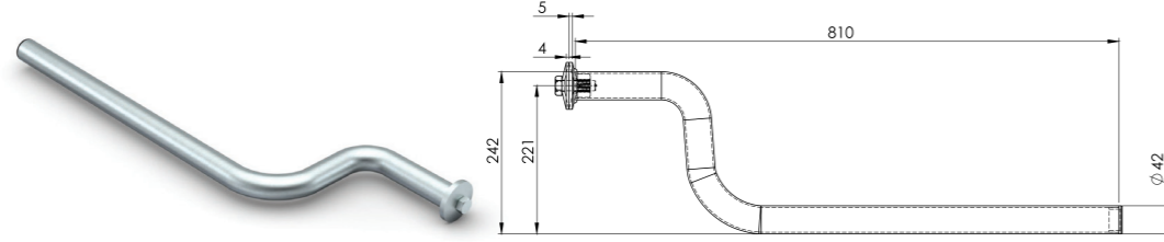
ÇAMURLUK BORUSU BÜKÜMLÜ GALVANİZ - DALDIRMA GALVANİZ 810MM MUDGUARD'S PIPE HOT DIP GALVANIZED (HDG) - (ZP)
