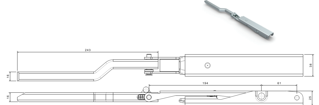
ORTA BABA MEKANİZMA SOL / MIDDLE PILLAR MECHANISM LEFT
