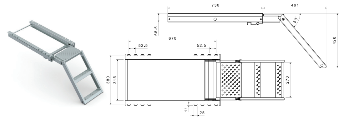
2 BASAMAKLI PLATFORMLU MERDİVEN 2 STEPS PLATFORM LADDER
