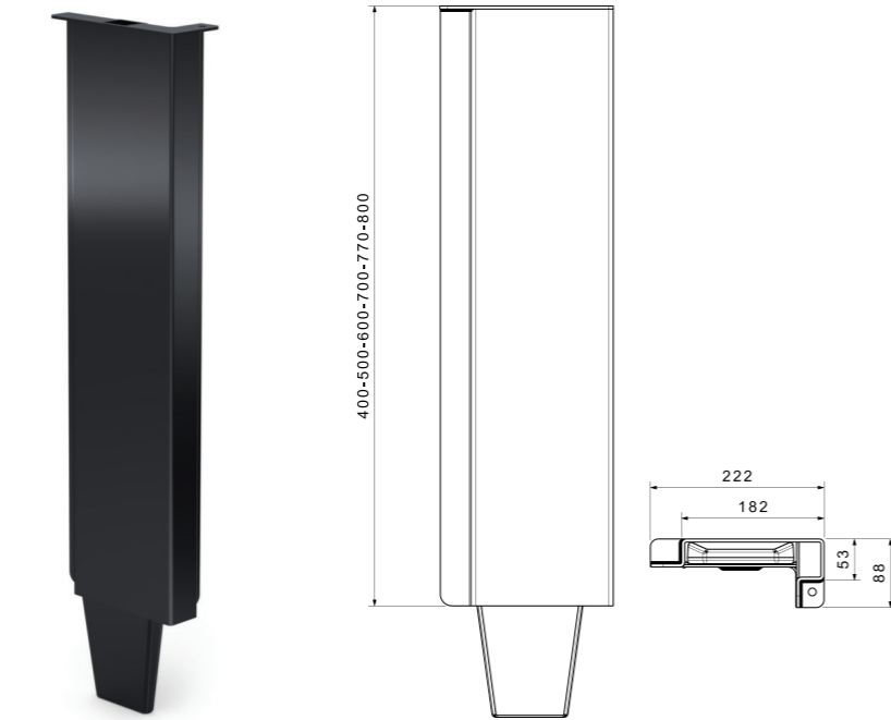
MEKANİZMASIZ ARKA BABA KATAFOREZLİ SOL UNMECHANISM REAR PILLAR LEFT KTL
