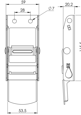
KÜÇÜK BRANDA TOKASI KROM - GALVANİZ SMALL TARPAULIN BUCKLE (SS) - (ZP)
