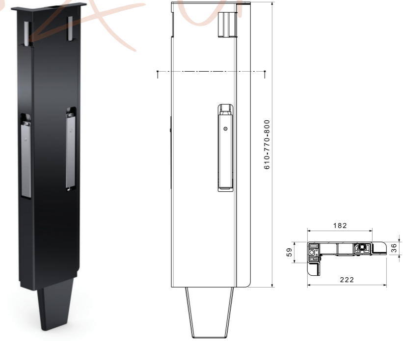
DİKEY KİLİT ARKA BABA KATAFOREZLİ SAĞ VERTICAL LOCK REAR PILLAR RIGHT KTL
