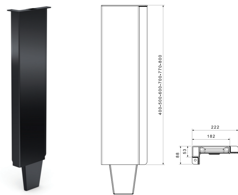
MEKANİZMASIZ ARKA BABA KATAFOREZLİ SAĞ UNMECHANISM REAR PILLAR RIGHT KTL
