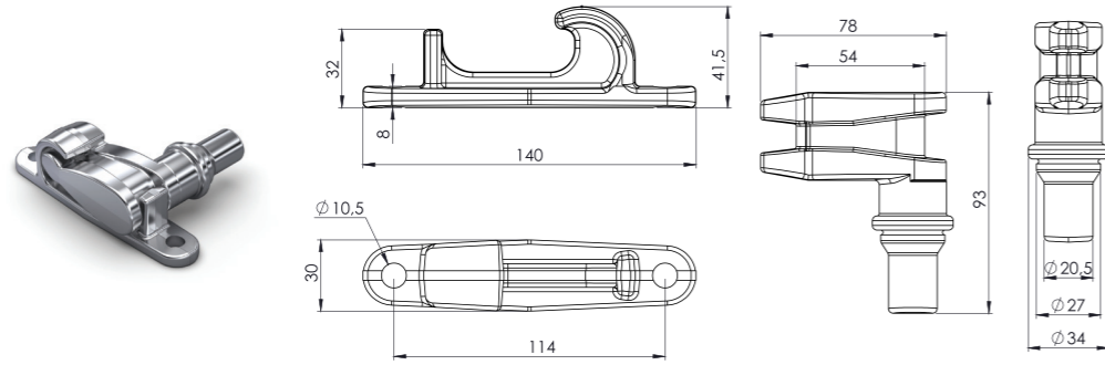
UNITNOVA TEK YÖN KANCA TAKIMI Ø27 CAM AND KEEPER FOR LOCK Ø27 (SS)
