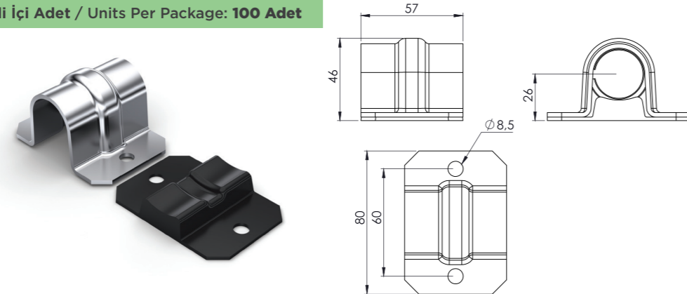
UNITNOVA EKO KÜÇÜK BORU YUVASI KROM Ø27 UNITNOVA SMALL GUIDE PLATE Ø27 (SS)
