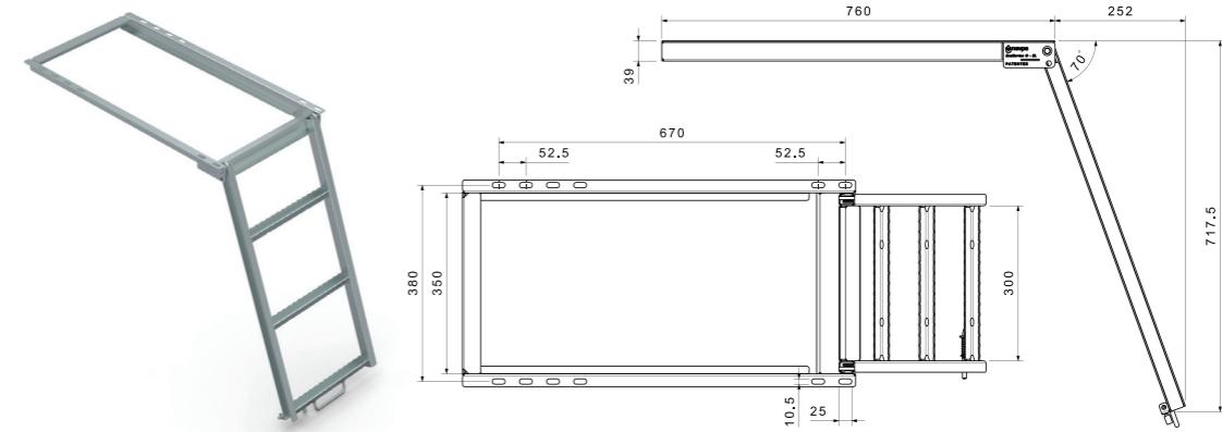
ECOSERIES 3 BASAMAKLI MERDİVEN DALDIRMA GALVANİZLİ ECOSERIES 3 STEPS LADDER HOT DIP GALVANIZED
