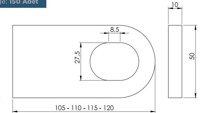
LAMA OVAL 50x10,5 - 50x11 - 50x11,5 - 50x12 / BRACKET
