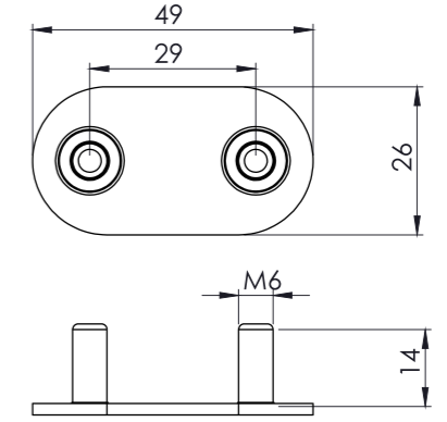
BRANDA TOKA SABİTLEME BRAKETİ KROM - GALVANİZ BUCKLE BRACKET (SS) - (ZP)
