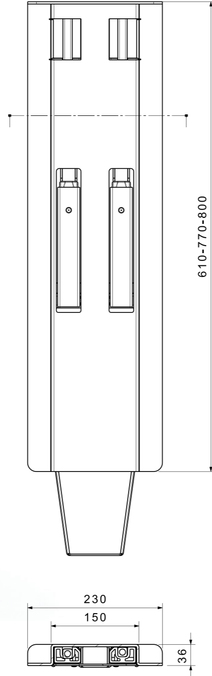
DİKEY KİLİT ORTA BABA KATAFOREZLİ VERTICAL LOCK MIDDLE PILLAR KTL
