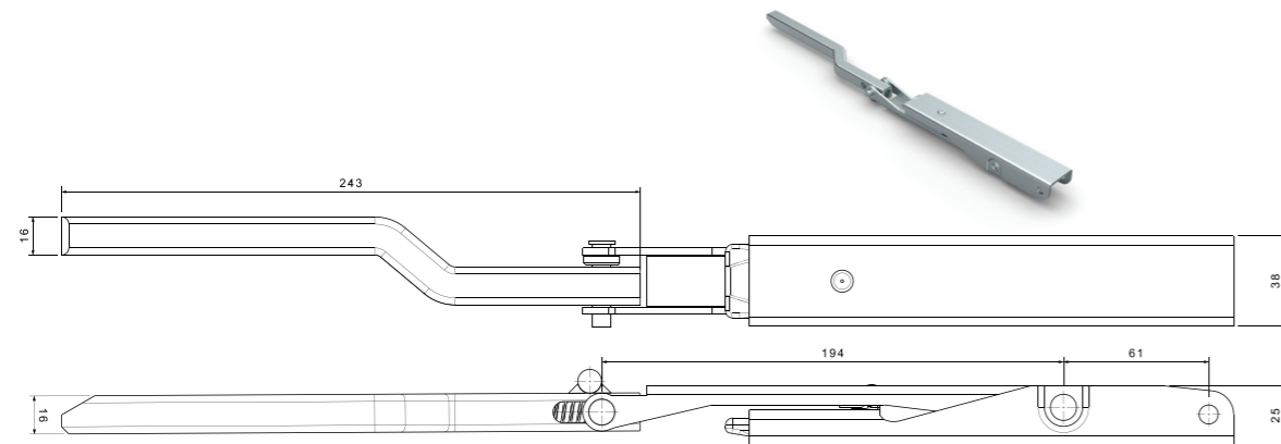
ORTA BABA MEKANİZMA SAĞ / MIDDLE PILLAR MECHANISM RIGHT
