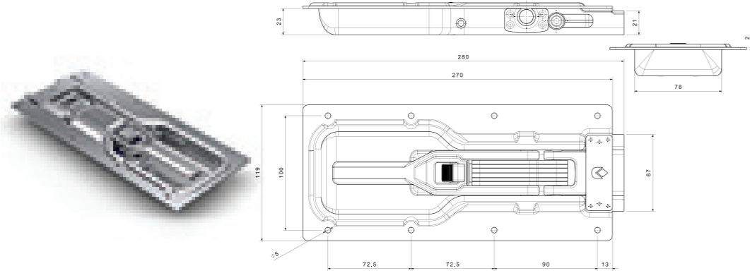
YENİ MODEL GÖMME KAPAK KİLİDİ LALE LOGOLU ADJUSTABLE SAFETY BOLT FASTENER
