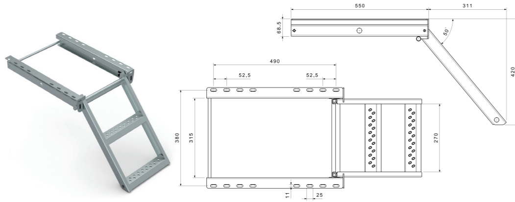
2 BASAMAKLI MERDİVEN / 2 STEPS LADDER
