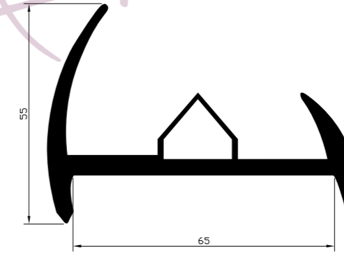
LP 65MM KAUÇUK PROFİL / RUBBER PROFILE 65MM
