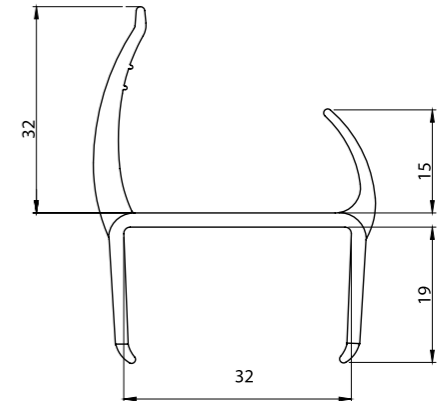
PVC PROFİL 32MM (SİYAH - BEYAZ , GRİ - BEYAZ) PVC PROFILE (BLACK - WHITE, GREY - WHITE)
