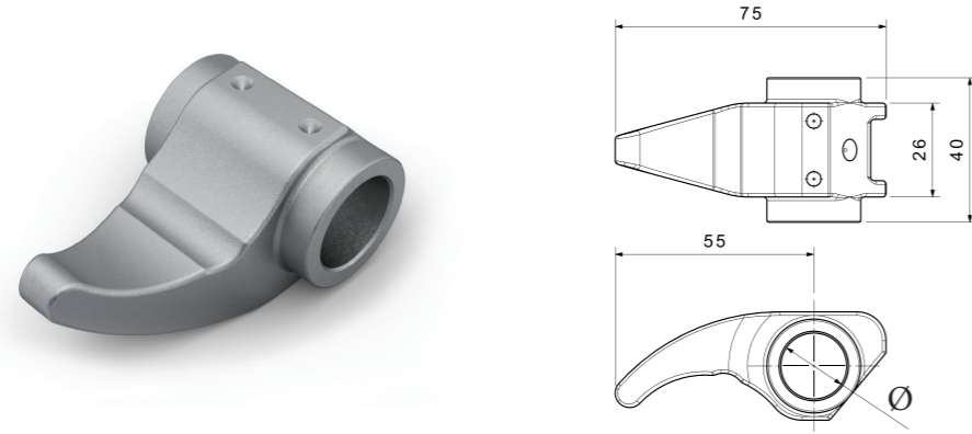
GİZLİ SİSTEM ARKA KAPI KİLİDİ ÜST TIRNAK (ÇİNKO+GEOMET) Ø18 - Ø16 LEADING CLAMPING CAM (ZINC AND GEOMET) Ø18 - Ø16
