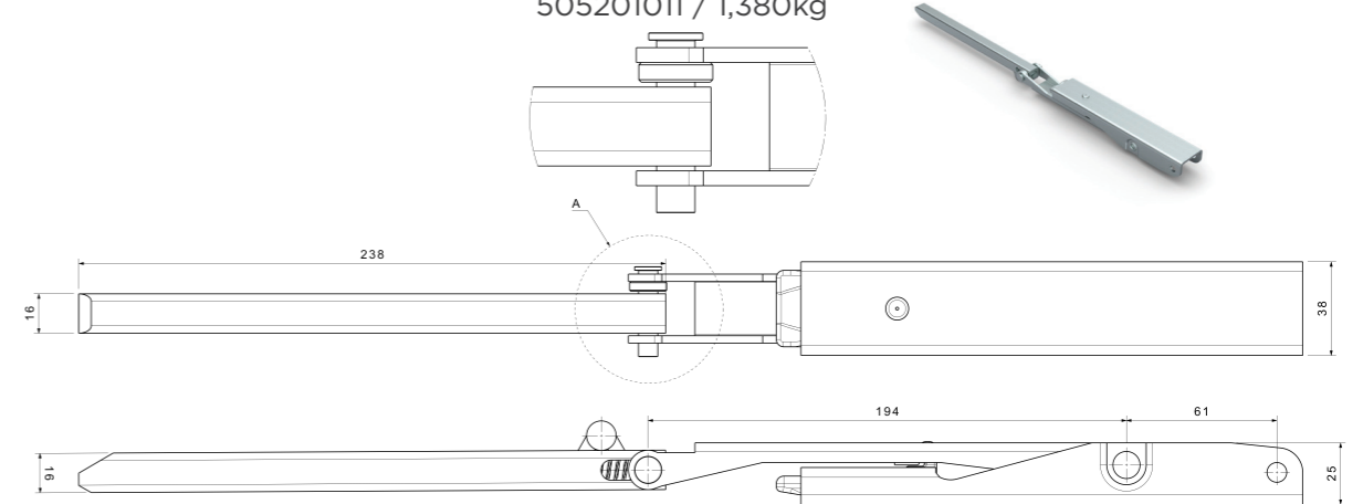
BABA DİKME KİLİT MEKANİZMASI 238MM - SOL MIDDLE PILLAR MECHANISM 238MM LEFT
