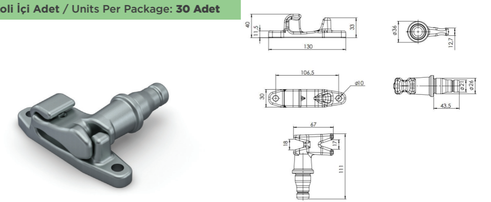
TEK YÖN ORTA BOY KANCA TAKIMI GALVANİZ Ø27 CAM AND KEEPER FOR LOCK Ø27 (ZP)
