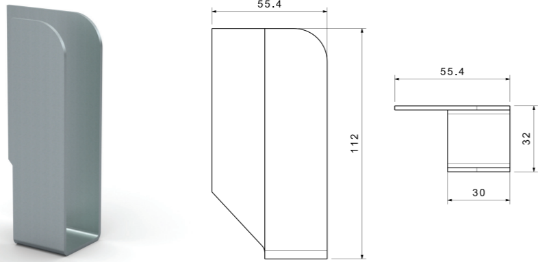
EKO KAYAR BABA TAHTALIK SACI SAĞ - SOL ECO SLIDING PILLAR SLAT STOWAGE LEFT AND RIGHT
