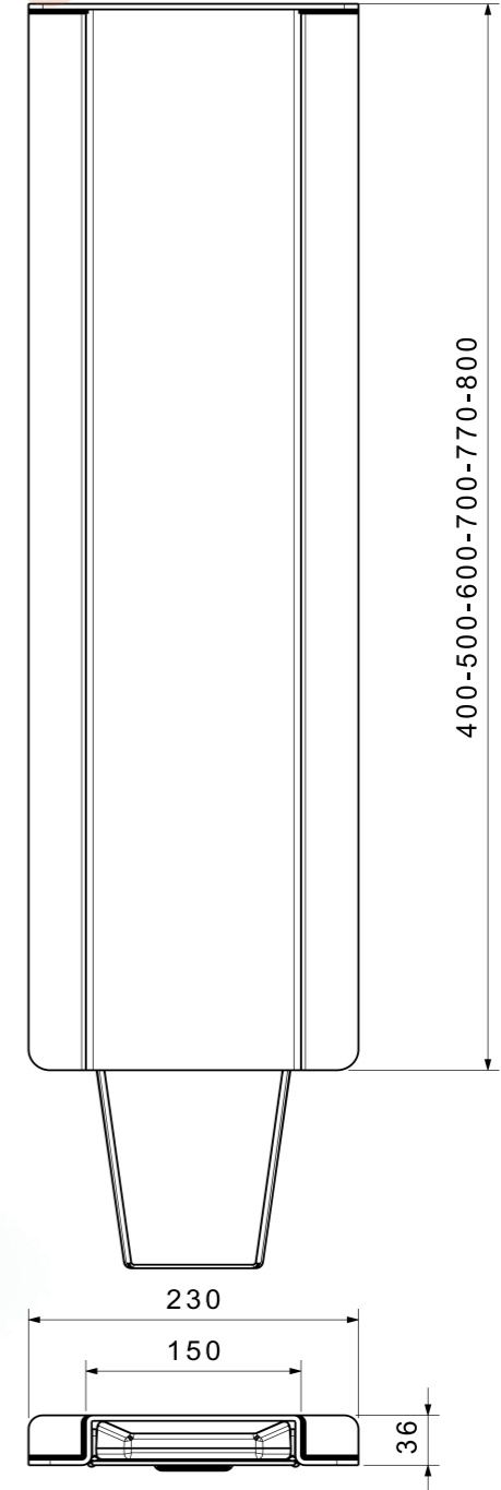
MEKANİZMASIZ ORTA BABA KATAFOREZLİ UNMECHANISM MIDDLE PILLAR KTL
