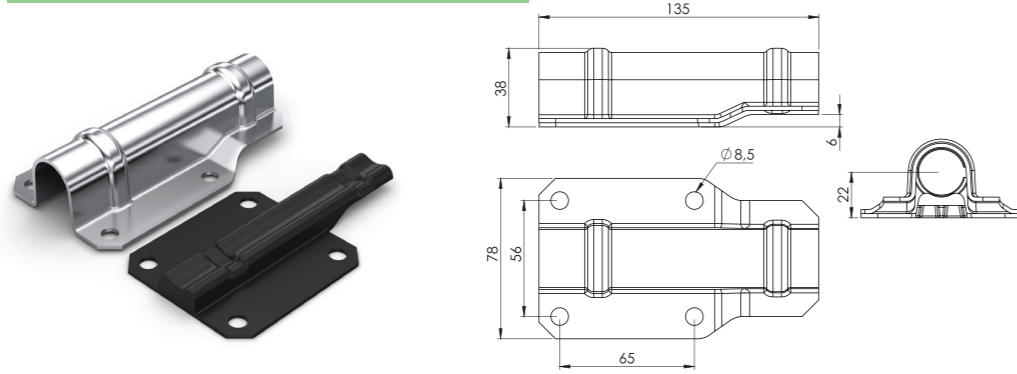
UNITNOVA EKO BÜYÜK BORU YUVASI KROM Ø22 UNITNOVA BIG GUIDE PLATE Ø22 (SS)
