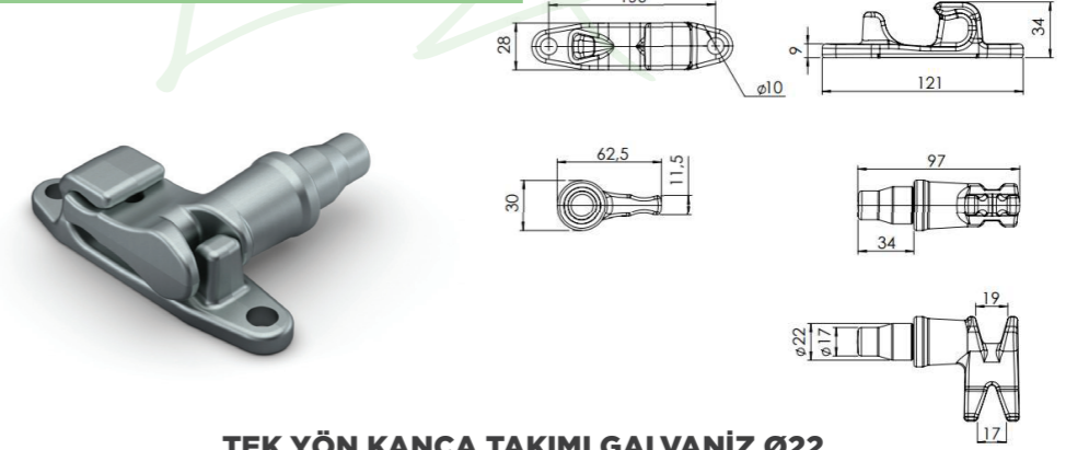
TEK YÖN KANCA TAKIMI GALVANİZ Ø22 CAM AND KEEPER FOR LOCK Ø22 (ZP)
