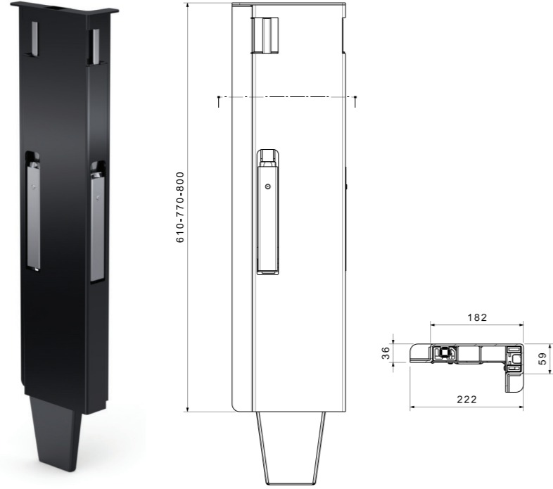
DİKEY KİLİT ARKA BABA KATAFOREZLİ SOL VERTICAL LOCK REAR PILLAR LEFT KTL
