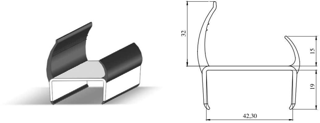
PVC PROFİL 42MM (SİYAH - BEYAZ , GRİ - BEYAZ) PVC PROFILE (BLACK - WHITE, GREY - WHITE)
