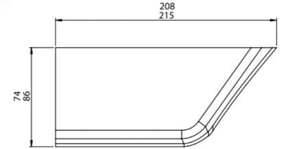
OVAL YARIM ETEK SACI / BRACKET
