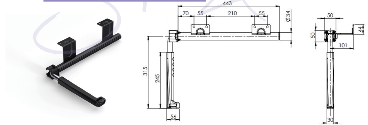
BOYALI ARKA KAPI TUTAMAĞI / DOOR HOLDER (PAINTED)
