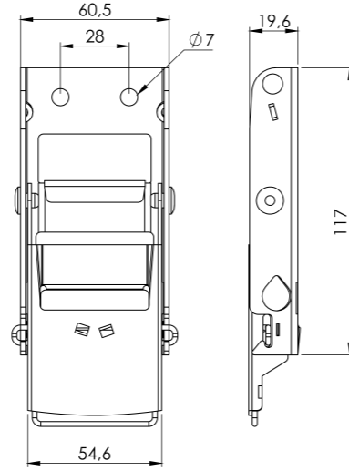
BRANDA TOKASI KİLİTLİ KROM TİP2 TARPAULIN BUCKLE WITH LOCK TYPE2 (SS)
