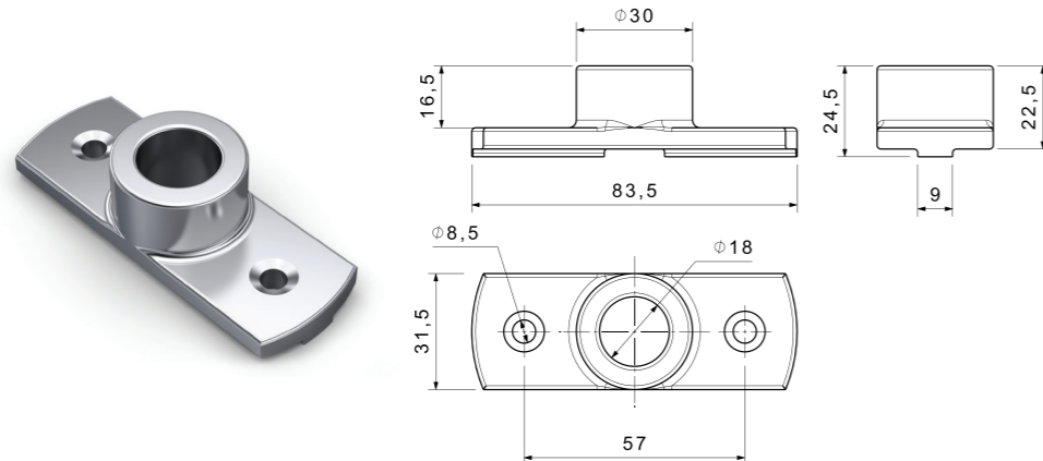
GİZLİ SİSTEM ALT PARÇASI (ÇİNKO+GEOMET) - (GALVANİZLİ) REAR DOOR LOCK UNDER BRACKET
