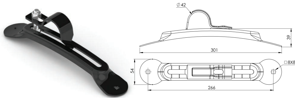
ÇAMURLUK KELEPÇESİ KÜÇÜK BOYALI SMALL MUDGUARD'S CLAMP (PAINTED)
