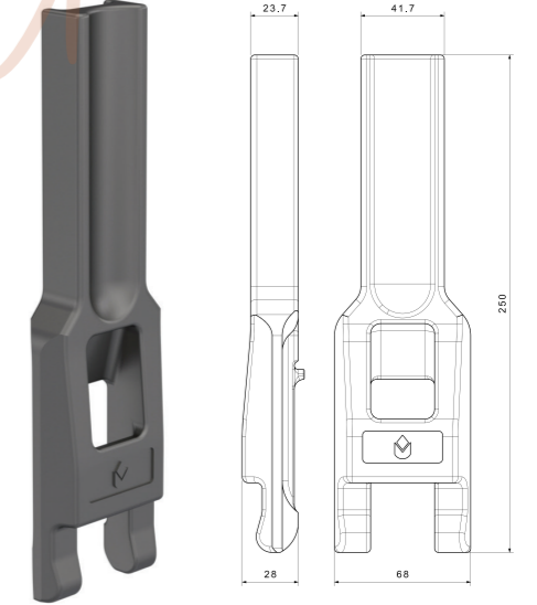
LALE SERİSİ KIRILIR BABA FÜZESİ TULIP SERIES MIDDLE PILLAR - ROOF CONNECTION PARTS
