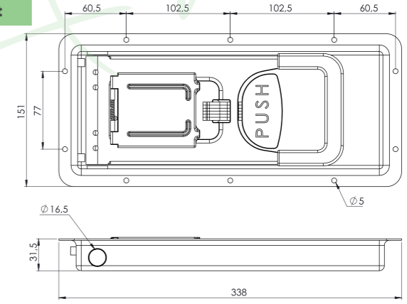
BÜYÜK GÖMME KİLİT KROM / RECESSED DOOR LOCK WITH KEY (SS)
