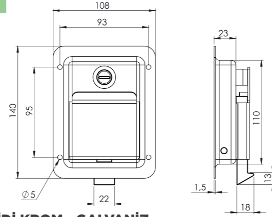
GÖMME KABİN KİLİDİ KROM - GALVANİZ RECESSED HANDLE LOCK WITH KEY (SS) - (ZP)
