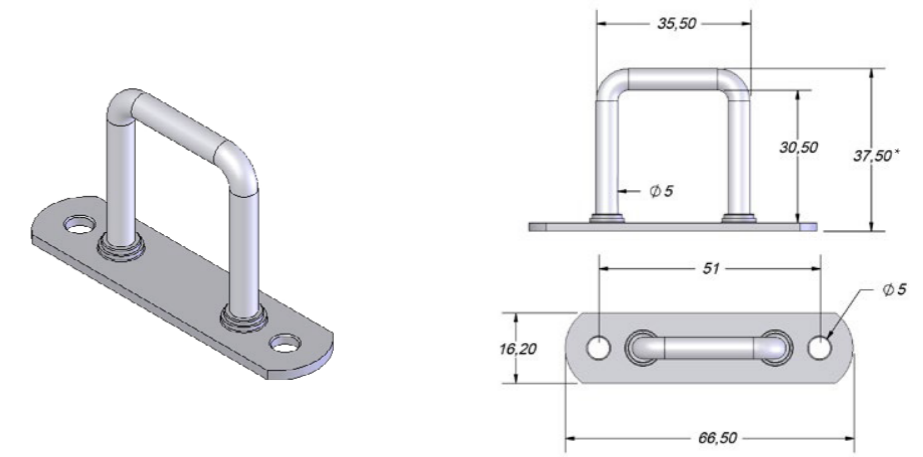
BRANDA KANCASI GALVANİZ 37.5MM ve 45MM / TARPAULIN HOOK
