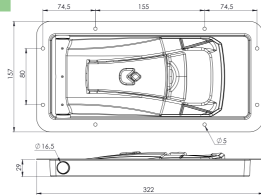
UNITNOVA GÖMME KİLİT 29MM KROM Ø16 UNITNOVA RECESSED DOOR LOCK WITH KEY 29 MM Ø16 (SS)
