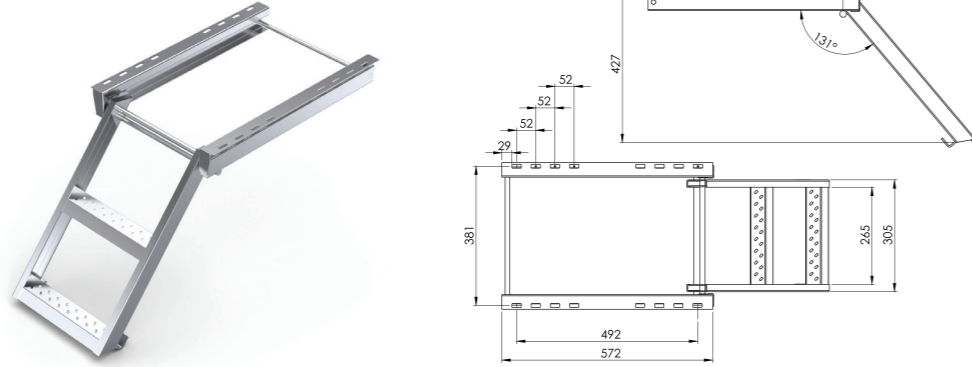
2 BASAMAKLI ARKA MERDİVEN GALVANİZ - DALDIRMA GALVANİZ 2 STEPS REAR LADDER HOT DIP GALVANIZED (HDG) (ZP)
