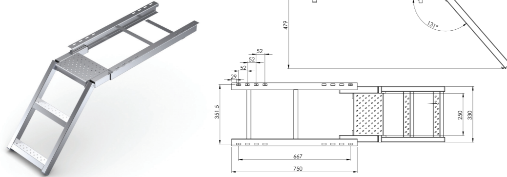
PLATFORMLU ARKA MERDİVEN GALVANİZ - DALDIRMA GALVANİZ READ LADDER WITH PLATFORM (ZP)
