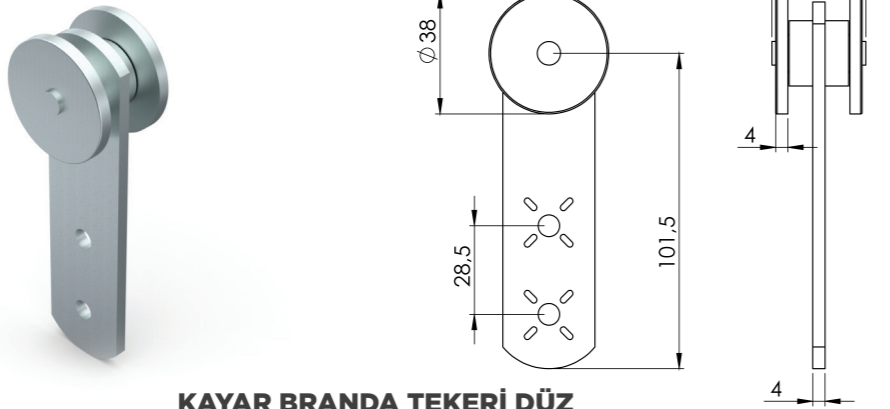
KAYAR BRANDA TEKERİ DÜZ SLIDING TARPAULIN ROLLER FLAT
