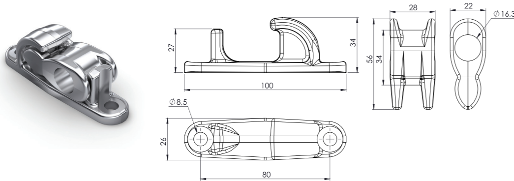
UNITNOVA PASLANMAZ KANCA TAKIMI Ø16 CAM AND KEEPER FOR LOCK Ø16 (SS)
