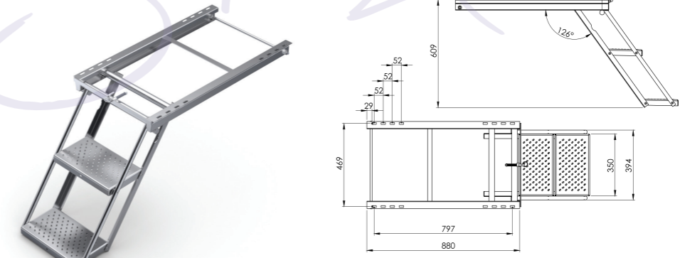
GENİŞ BASAMAKLI MERDİVEN DALDIRMA GALVANİZ WIDE STEP LADDER HOT DIP GALVANIZED (HDG) (ZP)
