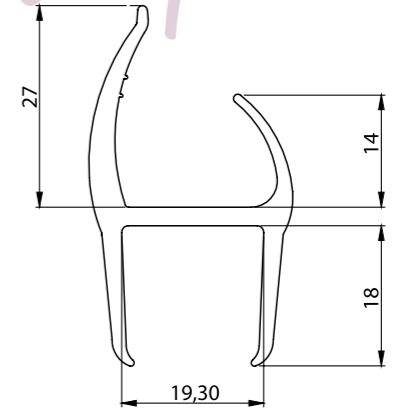
PVC PROFİL 19MM (SİYAH - BEYAZ , GRİ - BEYAZ) PVC PROFILE (BLACK - WHITE, GREY - WHITE)
