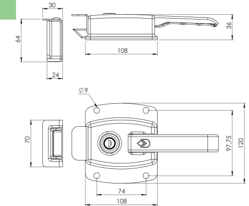
DONDURMA KİLİDİ KROM / HANDLE LOCK (SS)
