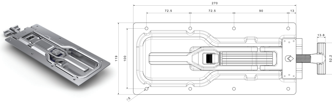
YENİ MODEL GÖMME KAPAK KİLİDİ + T PARÇASI 60MM MONTAJLI ADJUSTABLE SAFETY BOLT FASTENER + T PIECE 60MM
