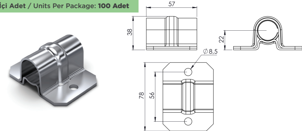
UNITNOVA KÜÇÜK BORU YUVASI KROM Ø22 UNITNOVA SMALL GUIDE PLATE Ø22 (SS)
