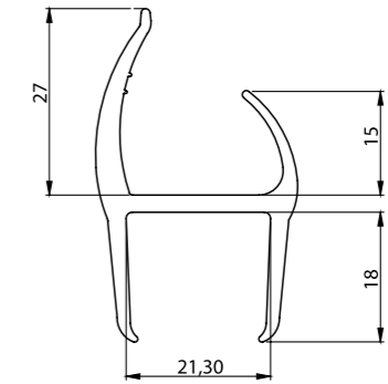
PVC PROFİL 21MM (SİYAH - BEYAZ , GRİ - BEYAZ) PVC PROFILE (BLACK - WHITE, GREY - WHITE)
