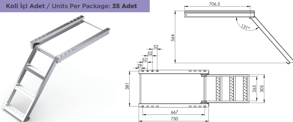
3 BASAMAKLI ARKA MERDİVEN GALVANİZ - DALDIRMA GALVANİZ 3 STEPS REAR LADDER (ZP)
