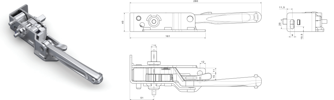
YENİ BRANDA GerdİRME MEKANİZMASI KARE & U ADAPTÖRLÜ DÜZ KOLLU DALDIRMA GALVANİZLİ / RATCHET TYPE NEW HOT DIP GALVANIZED
