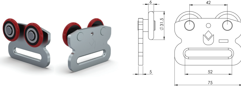
KAYAR BRANDA ÇİFT TEKER SLIDING TARPAULIN DOUBLE ROLLER
