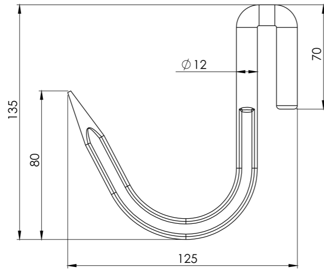
YAN ET KANCASI KROM / MEAT HOOK (SS)
