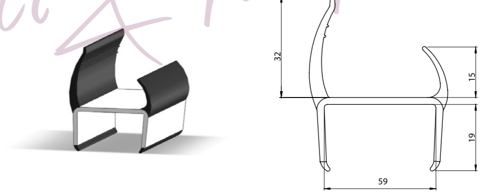
PVC PROFİL 60MM (SİYAH - BEYAZ , GRİ - BEYAZ) PVC PROFILE (BLACK - WHITE, GREY - WHITE)
