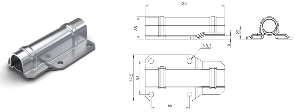
UNITNOVA BÜYÜK BORU YUVASI KROM Ø22 UNITNOVA BIG GUIDE PLATE Ø22 (SS)
